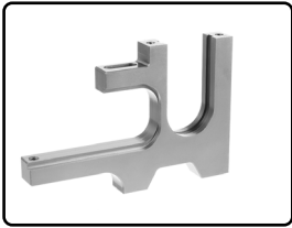
C-00180-605 Motor Bulkhead - V2 - Aluminium - Composite - 1 pc
