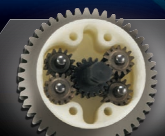
Planetary Differential
