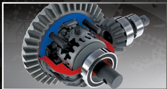
MAXX® DUTY DRIVETRAIN
