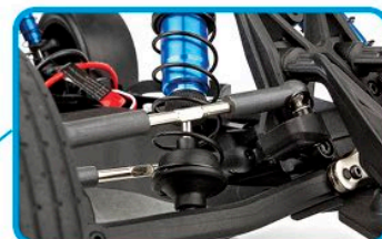
Rugged steel turnbuckles for adjustable camber and front toe-in
