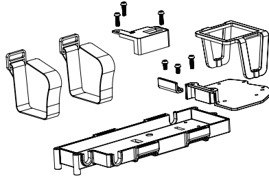
500405768 Akkuhalter Set Battery holder
