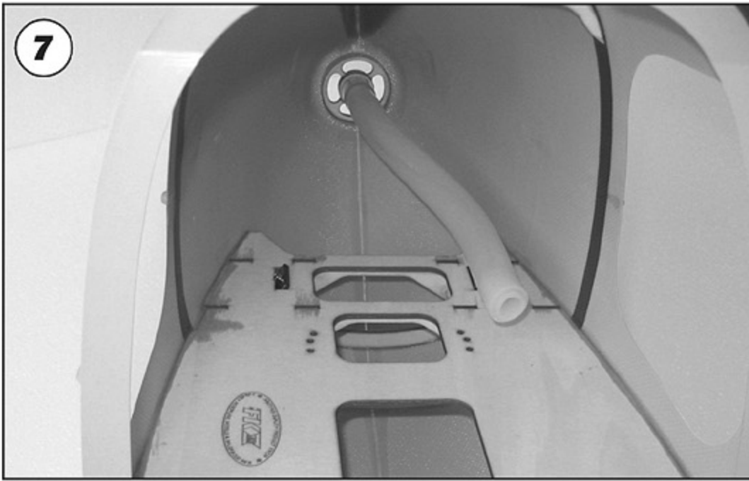
7 Connect the exhaust tube to the exhaust mount and tie them with nylon strap. 將排煙導管接上排煙管座，並以束帶束緊固定。
