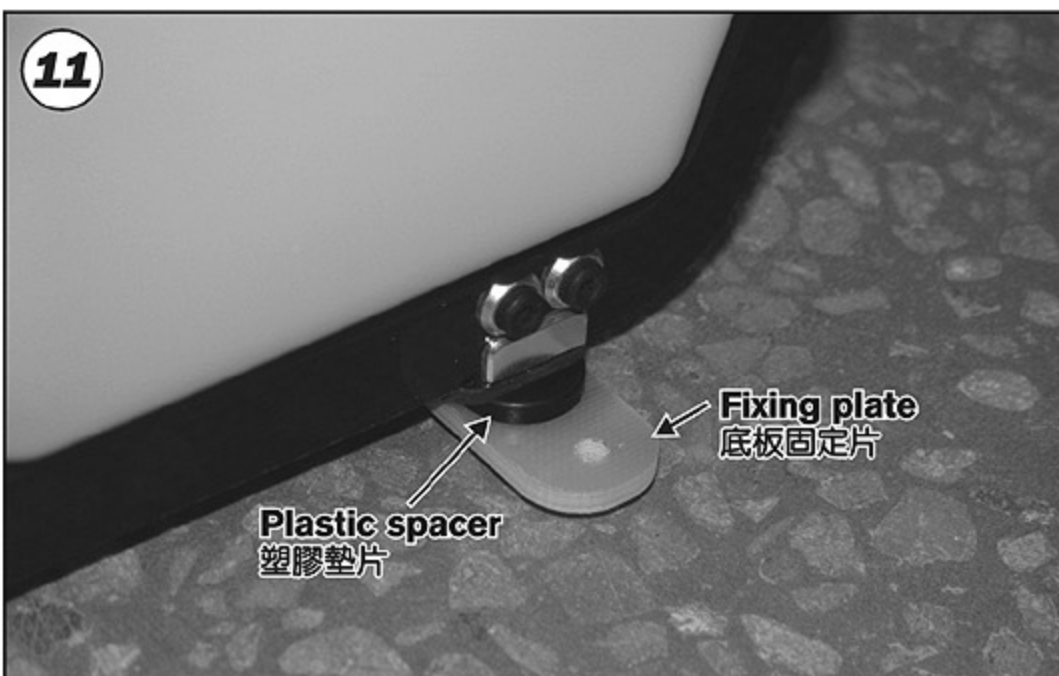
11 First remove the original 600N landing skids. Assemble the plastic spacers and the fixing plate in the back of the bottom plate to raise it. 先將600N的原腳架拆除，於碳纖底板後方以塑膠墊片和底板固定片將碳纖底板架高。
