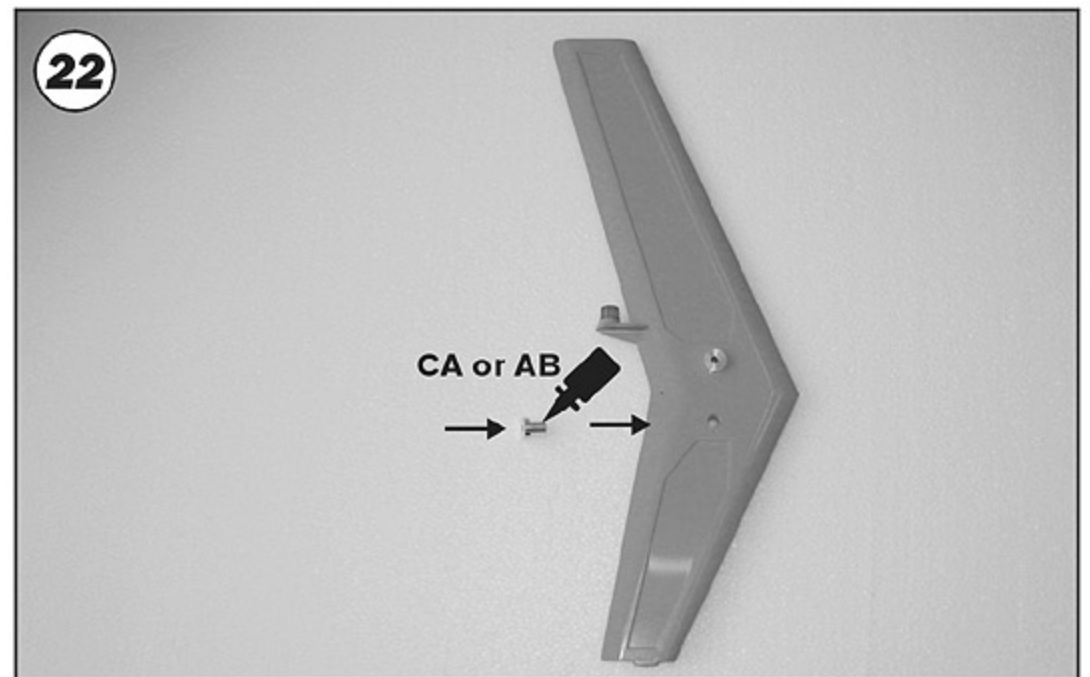
22 Apply some CA or AB glue on the aluminum inserts and insert into the vertical stabilizer from the right side. 將垂直翼固定鋁套點上CA或AB膠後，由右側壓入垂直翼。
