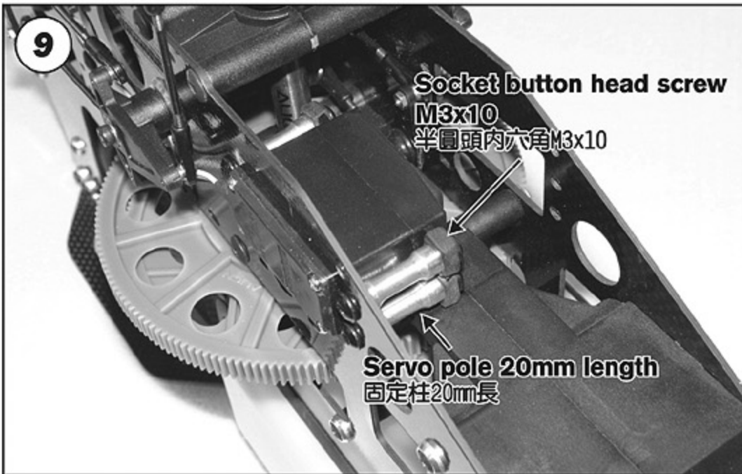
9 Raise the elevator servo by ELEV servo poles and screw it for preventing any interference caused by the fuselage. 如圖示，將ELEVATOR伺服器以隨附的固定柱(20mm長)架高固定，可避免與機殼干涉。
