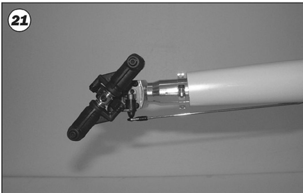
21 Reinstall the tail case as the standard assembly. Fasten the ball link in a proper position, and then to the linkage ball. 將尾齒箱組依標準方式裝回，鎖上連桿頭調整至適當長度後，壓入球頭。
