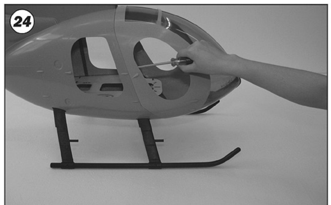
24 Fasten the canopy with 6pcs round head tapping screws T3x10. 機頭罩以6pcs圓頭十字螺絲T3x10鎖附固定。
