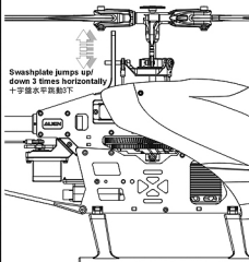
Swashplate jumps up and down 3 times horizontally represents successful initialization.
